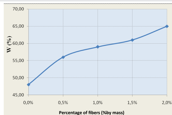
Figure 3: Variation of water absorption of mortar of plaster in function of the percentage by mass of fibers.
