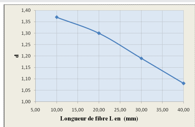
Figure 6: Variation of density of mortar of plaster in function of different fiber lengths.
