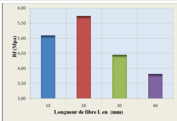
Figure 8: Variation in the compressive strength of plaster mortar as a function of different fiber lengths.
