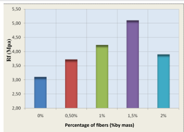
Figure 5: Variation of the flexural strength of plaster mortar as a function of the percentage by mass of fibers.
