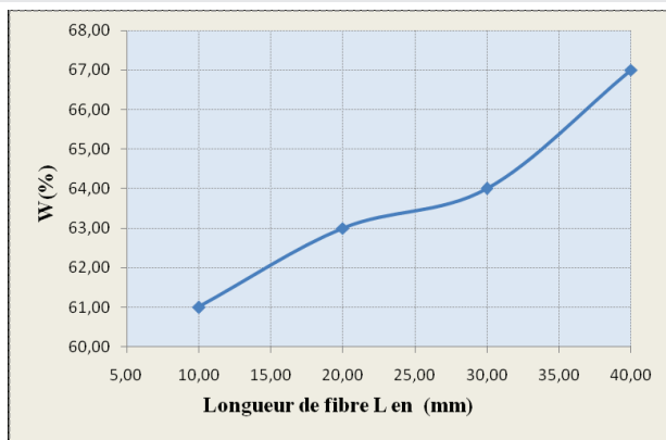
Figure 7: Variation of the water absorption of plaster mortar as a function of different fiber lengths.
