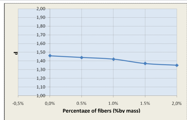
Figure 2: Variation of density of mortar of plaster in function of the percentage by mass of fibers.
