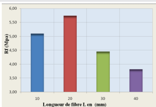
Figure 9: Variation of the flexural strength of mortar plaster in function of different fiber lengths.
