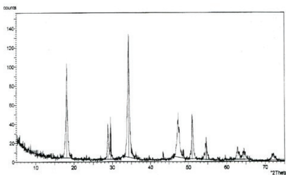
Figure 1: Diffractogramme of the powder lime by X-ray.
