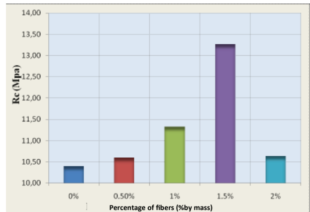
Figure 4: Variation of compressive strength of mortar cast according to the mass percentage of fibers.
