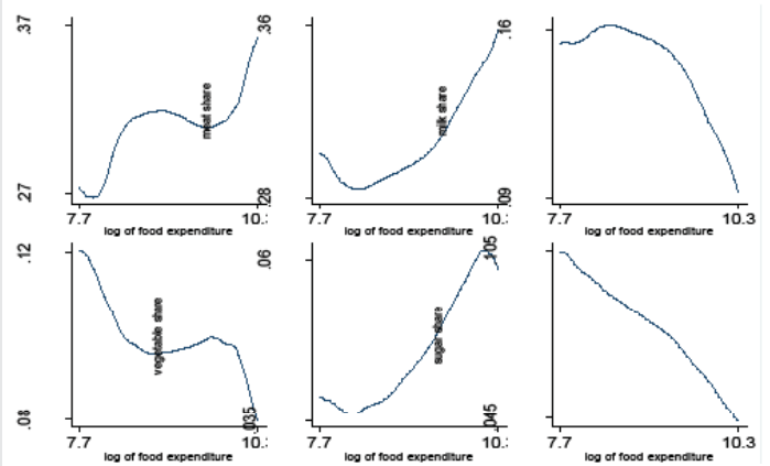
Figure 1: Explain the non-parametric Engel Curve for 6 groups of food share.
